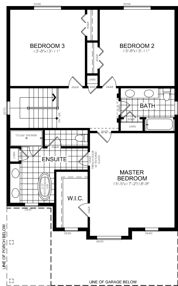
UPPER FLOOR PLAN FLOOR AREA = 1170 SQ.FT.
