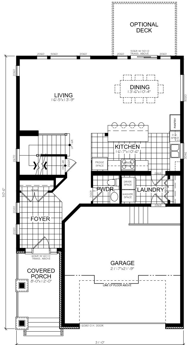
MAIN FLOOR PLAN FLOOR AREA = 940 SQ.FT.
