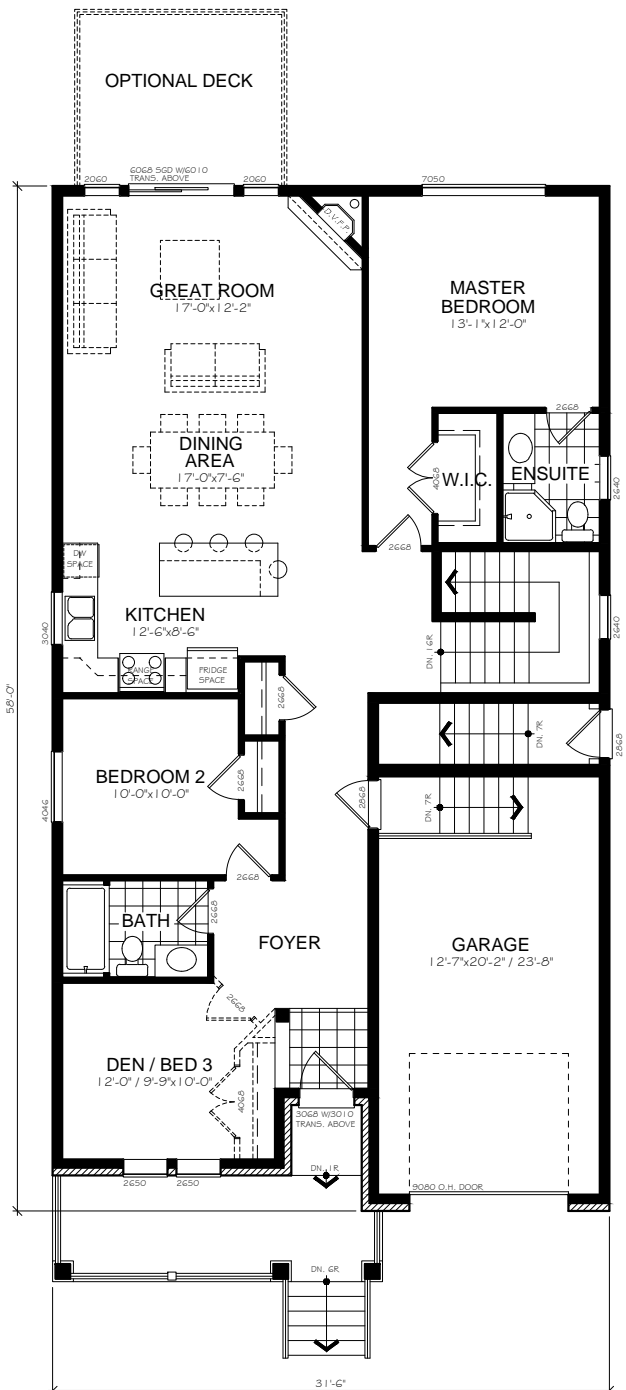
MAIN FLOOR PLAN 1395 SQ.FT.
