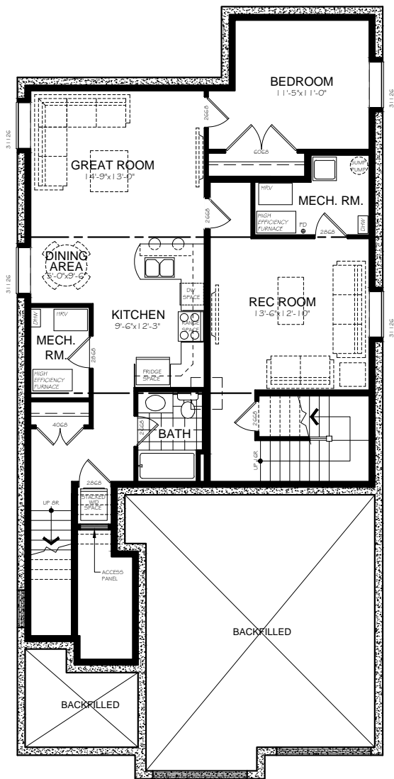
BASEMENT PLAN
