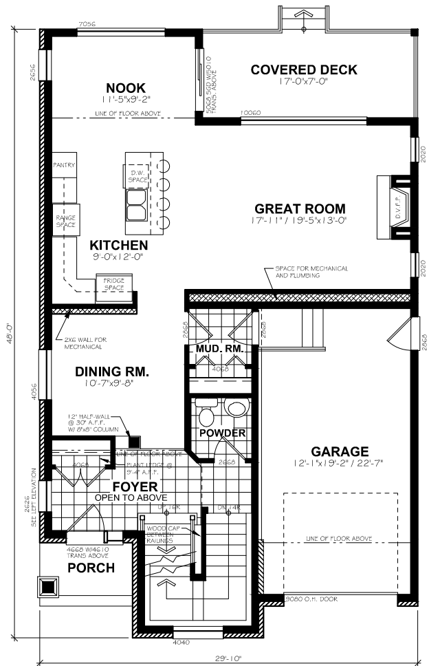
MAIN FLOOR PLAN 930 SQ.FT.
