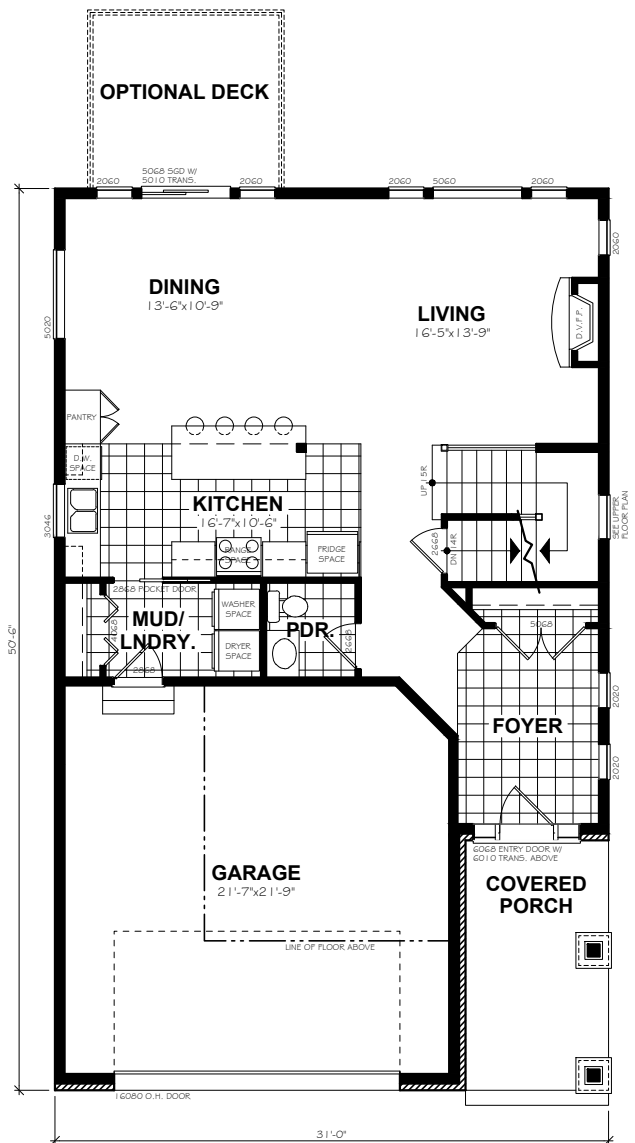
MAIN FLOOR PLAN 940 SQ.FT.
